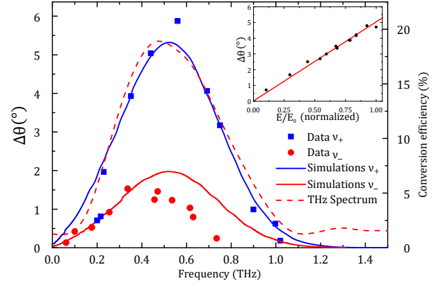
Figure 3: Polarization rotation angle as a function of the measured frequency. Comparison of experimental oscillatory signals as a function of their frequency for the High Frequency (squares) and the Low Frequency (dots) modes for a 400 nm wavelength. Simulations based on the numerical evaluation of time integration of Eq. (4) are displayed in solid lines. For comparison, the experimental THz spectrum is shown in dashed line. Inset: Polarization rotation angle for the high frequency oscillation versus the THz electric field strength for \alpha_{in} = 9.3^{\circ} and \lambda_o = 400 nm in the front-side configuration.
