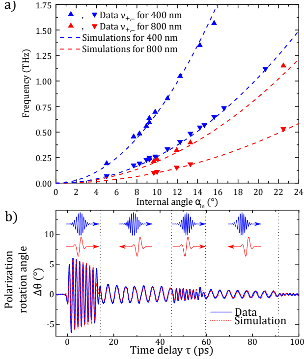
Figure 2: (a) Measured frequencies as a function of the probe's incidence angle. Two different wavelengths \lambda_o = 400 nm (blue triangles) and \lambda_o = 800 nm (red triangles) are plotted as well as the predictions of our model for both wavelengths (dashed lines). (b) Comparison of the experimental and simulated polarization rotation transients for an angle \alpha_{in} = 10^{\circ} and \lambda_o = 400 nm. The corresponding oscillations frequencies are \nu_+ = 0.69 THz and \nu_- = 0.27 THz. Vertical dotted lines separate the regions with co- and counter-propagating pump and probe pulses.
