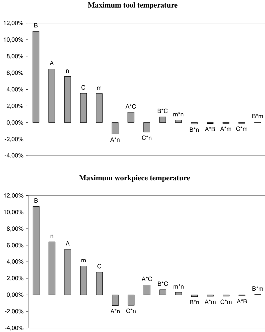
Fig. 6. Impact of Johnson-Cook parameters on the maximum temperatures.
