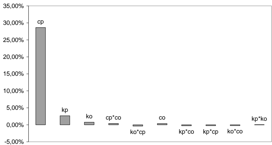
Fig. 12. Impact of thermal parameters on the cutting forces.
