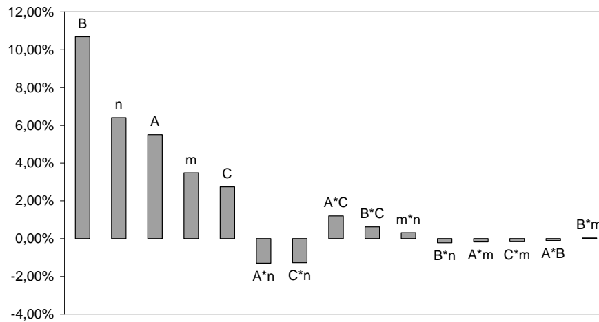
Fig. 6. Impact of Johnson-Cook parameters on the maximum temperatures.
