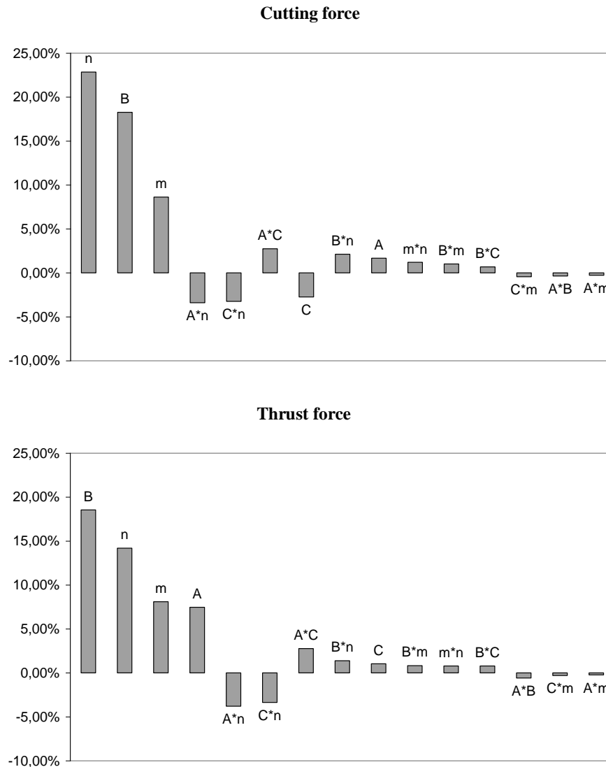
Fig. 8. Impact of Johnson-Cook parameters on the cutting forces.
