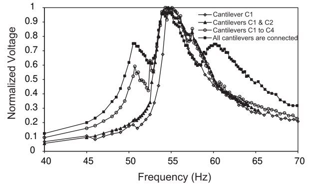
Fig. 9. Normalized output voltage at 1st resonance mode of different cantilever configurations, showing the frequency bandwidth as a function of the number of connected cantilevers.
