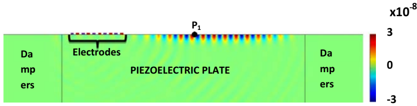
Fig. 2. Generation of SAW on IDT sensor ( t = 16 \times T = 800 ns).
