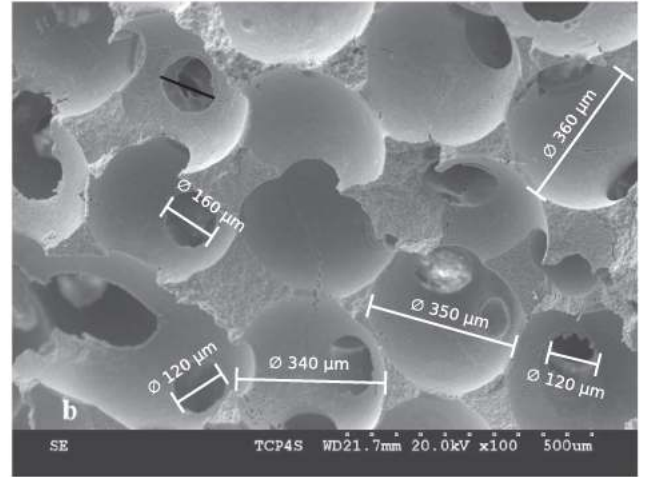
Fig. 2. SEM imaging of porous scaffold used as a reference for our numerical studies. Scaffold have average diameters of 350 \mu\text{m} and average diameters of interconnection of 150 \mu\text{m} .
