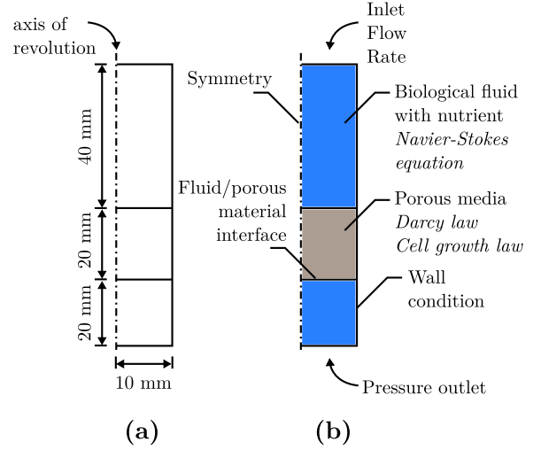
Fig. 4. Details of the macroscopic axisymmetric model: (a) dimensions (b) Boundary and numerical study conditions.
