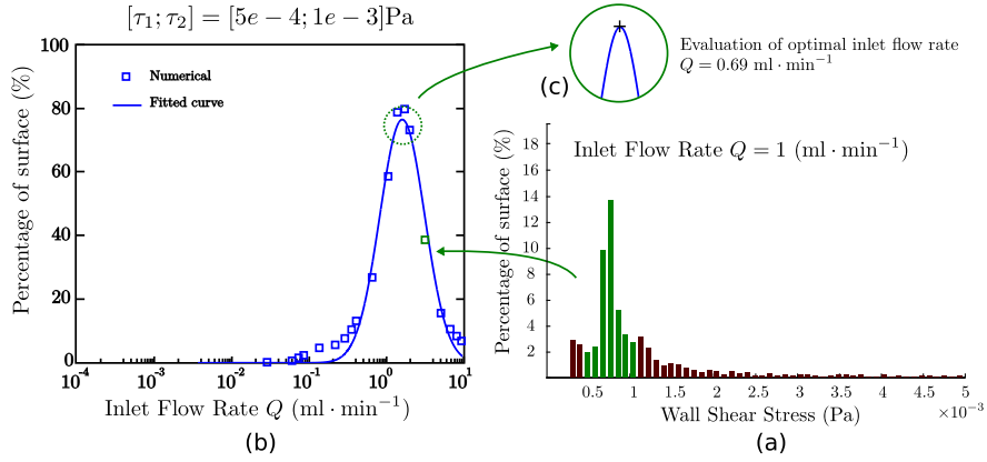
Fig. 7. (a) Histogram of WSS distribution for a given inlet flow rate, (b) Comparison between numerical data and log-normal function fitted, (c) Maximum of distribution and optimal inlet flow rate estimation.
