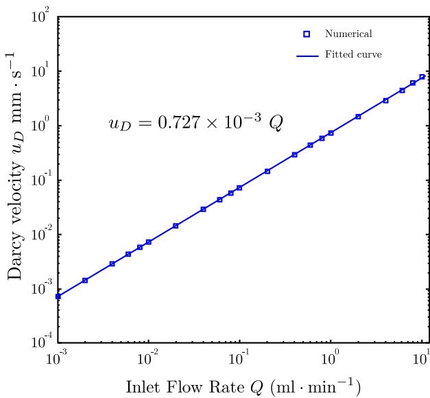
Fig. 8. Darcy velocity calculated in the REV as a function of flow rate Q .
