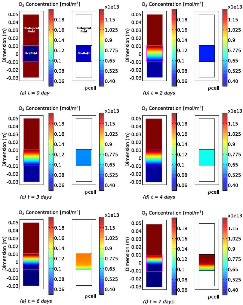
Fig. 9. Distribution of dioxygen concentration c_{O_2} and number of cells \rho_{cell} inside the bioreactor for several time-step (initial time to 7 days).
