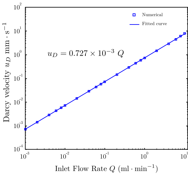
Fig. 8. Darcy velocity calculated in the REV as a function of flow rate Q .
