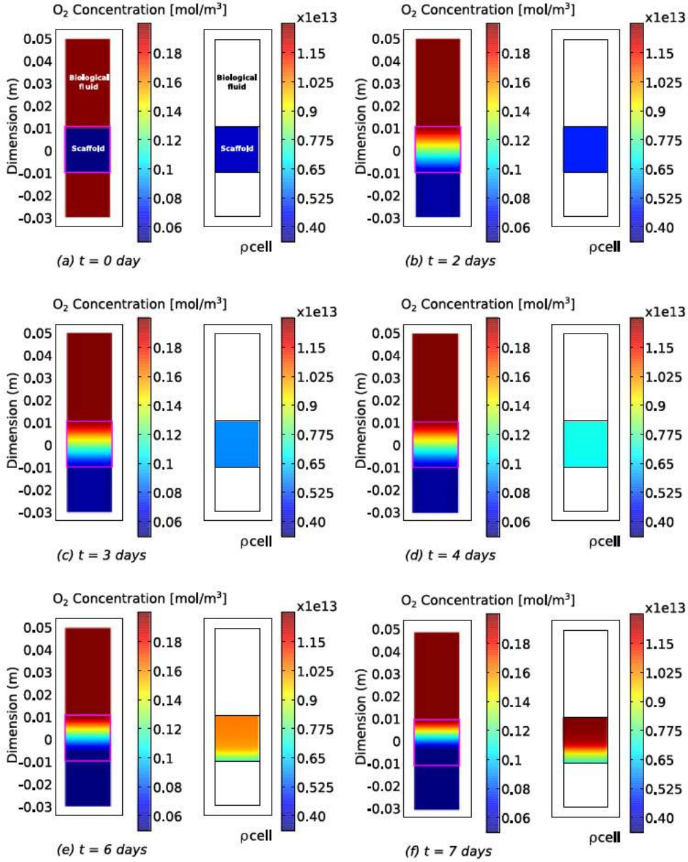
Fig. 9. Distribution of dioxygen concentration c_{O_2} and number of cells \rho_{cell} inside the bioreactor for several time-step (initial time to 7 days).
