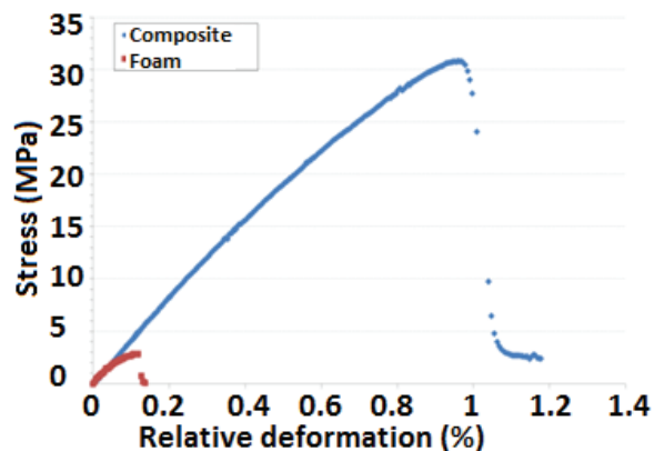
FIGURE 3. Bending tests of foam and the corresponding composite
