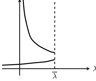
FIGURE 2. Illustration of Theorem 1.5 with h \gtrless 0
