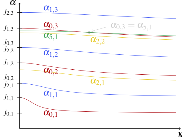
FIGURE 3. Graph of some \alpha_{k,\ell} .
