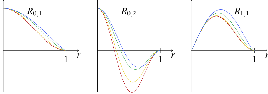
FIGURE 4. Graphs of R_{0,1} , R_{0,2} and R_{1,1} for \kappa = 0.1 (red), \kappa = 10 (orange), \kappa = 30 (green) and \kappa = 100 (blue).
