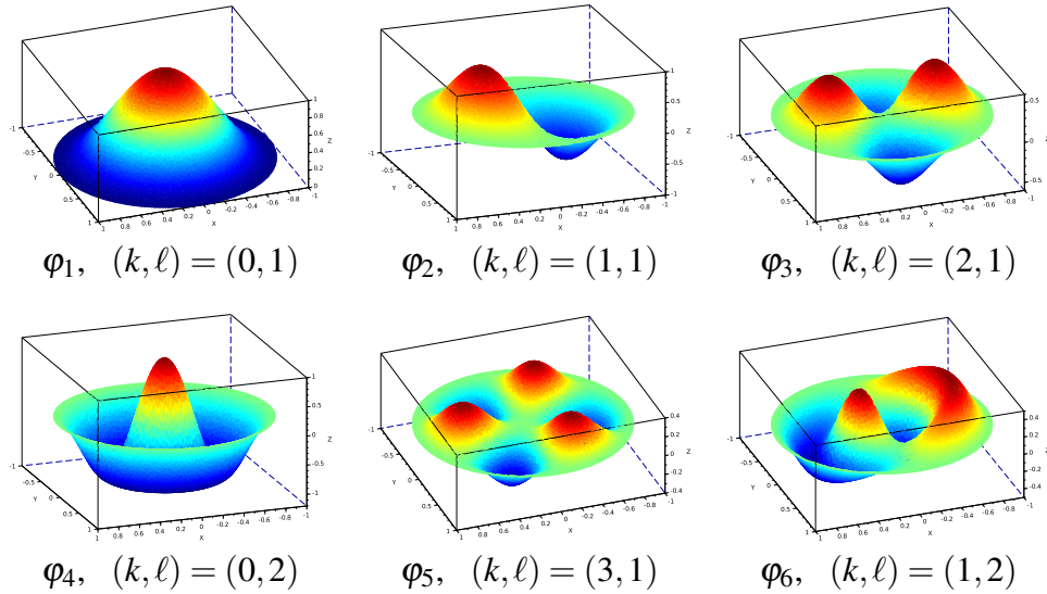
FIGURE 2. Graphs of the first eigenfunctions for v = -1 , mentioning the value (k, \ell) of Theorem 2 to which they correspond.
