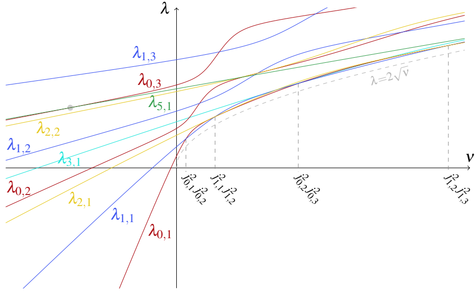
FIGURE 1. Curves of (v, \lambda) along which (1) possesses a nontrivial solution. The dot indicates where the graphs of \lambda_{0,3} (red) and \lambda_{5,1} (green) cross.
