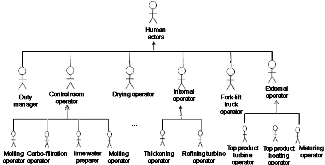
Figure 16. Some human actors identified relative to the dedicated mobility and cooperative task web services.
