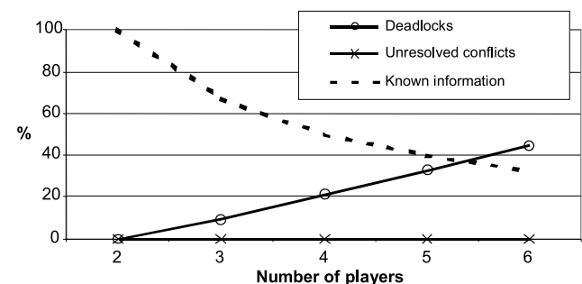
Fig. 6 Efficiency of the distributed multi-agent coordination mechanism
