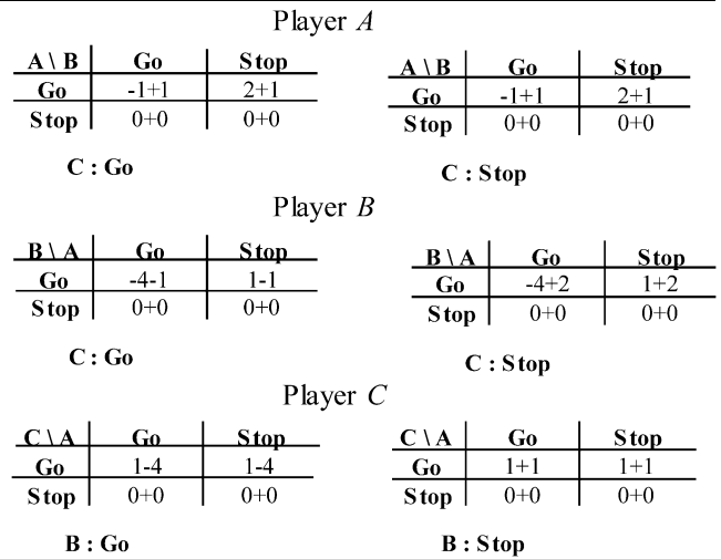
Fig. 11 Three-player matrices for each of the players
