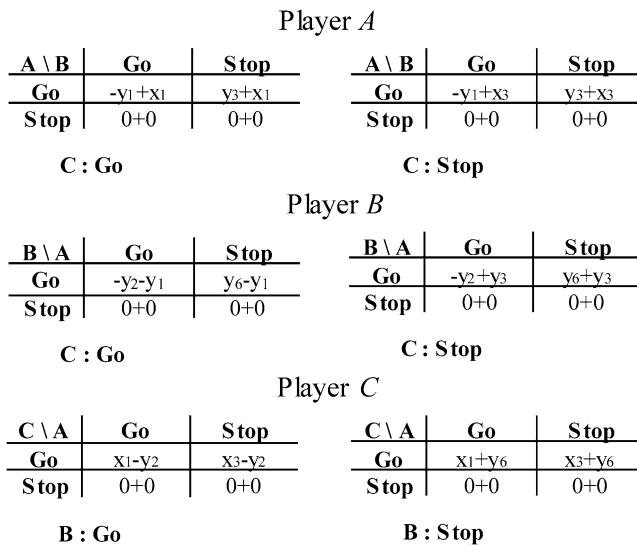
Fig. 10 The three-player matrices that model the situation for each of the three players
