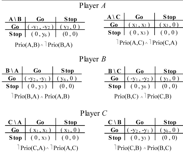
Fig. 9 The two-player matrices that model the situation for each of the three players
