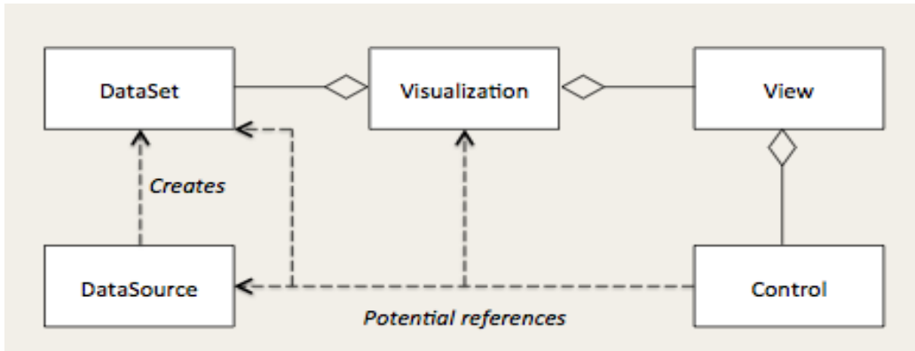
Fig. 5. Reference Model pattern [11]
