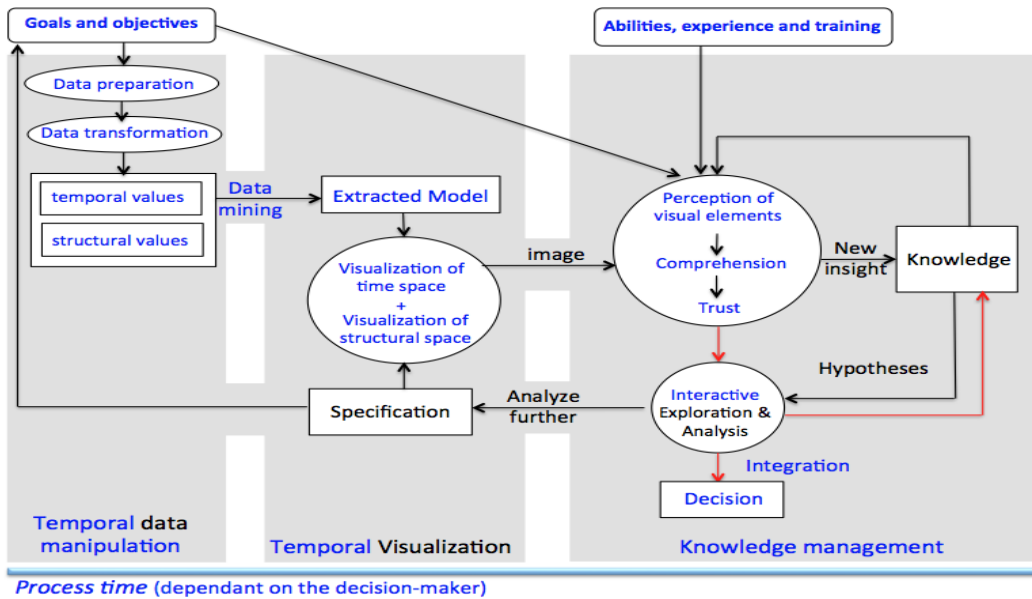
Fig. 11. Visual Analytics Model of Ltifi et al. [8]
