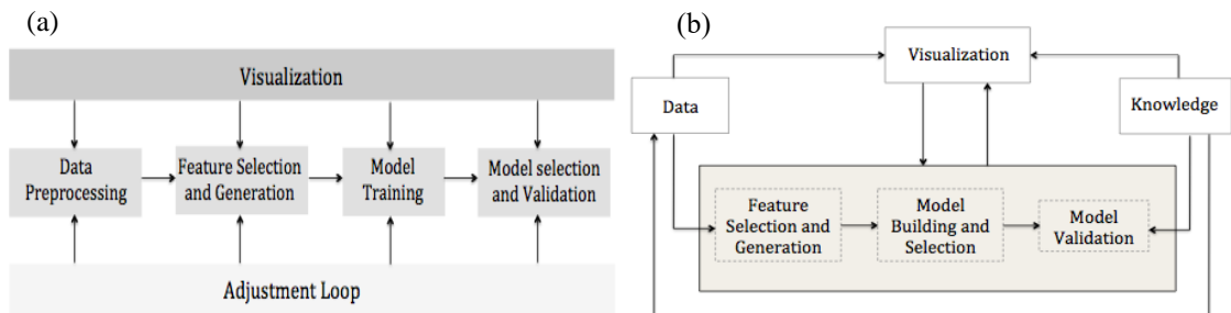
Fig. 13. (a) The specific predictive model of [70] and (b) The generalized version of [22]
