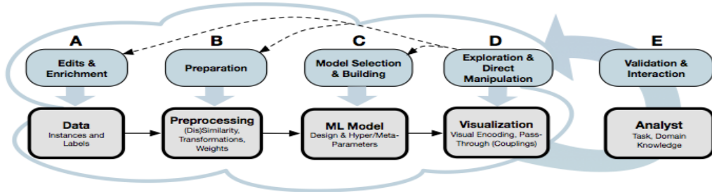
Fig. 14. Interactive Visual Analytics/Machine Learning of [29]
