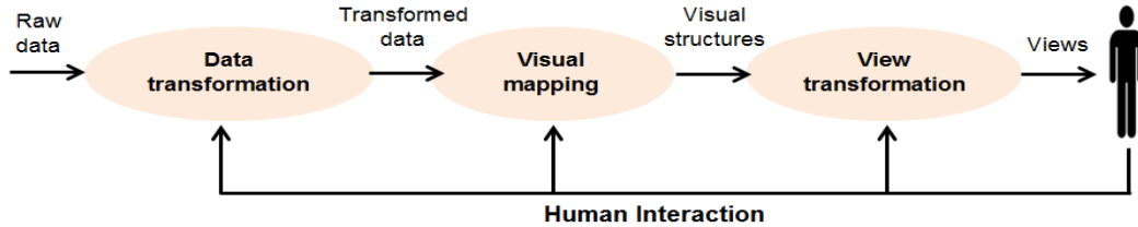
Fig. 2. Information Visualization reference model [1]
