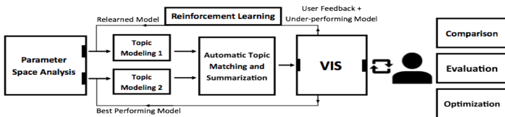
Fig. 15. The progressive learning model of [72]
