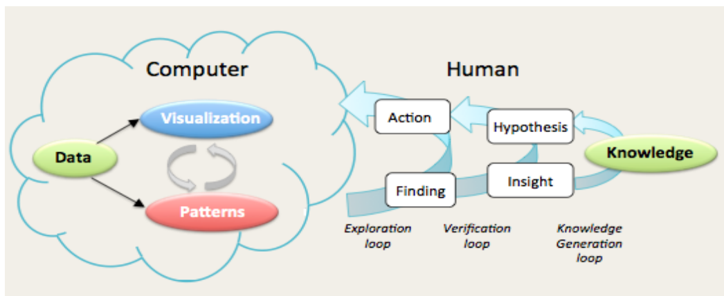
Fig. 10. Visual Analytics Model of Sacha et al. [7]
