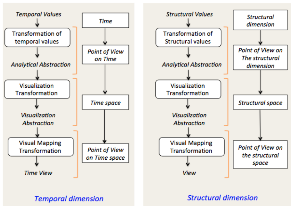
Fig. 4. Visualization process of temporal data [32]
