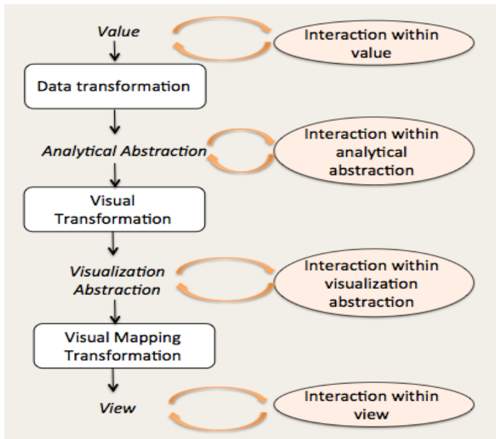
Fig. 3. Data State Reference Model [6]
