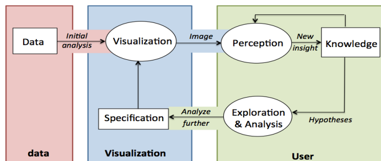
Fig. 3. The Generic Visual Analytics process (inspired from [11])
