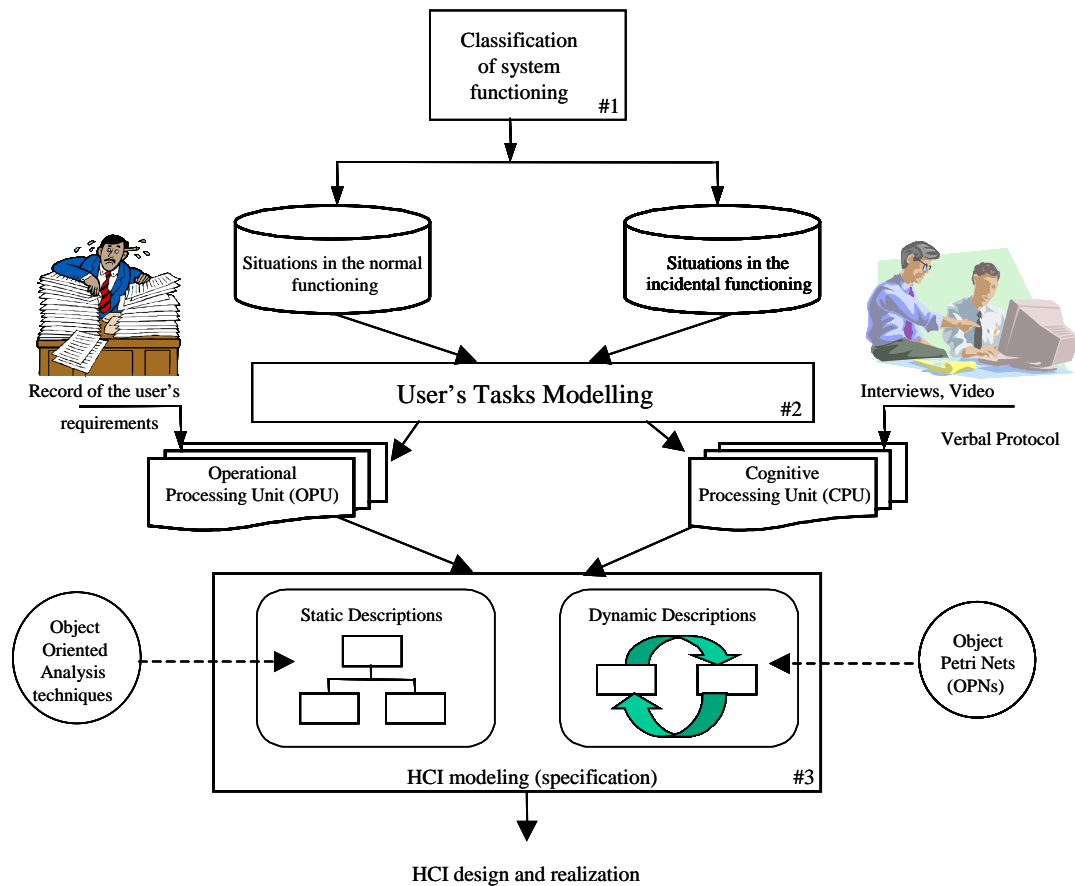
Fig. 2. Modelling process
