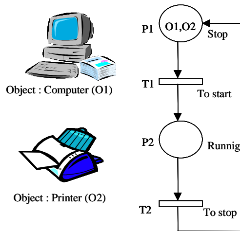
Fig 3. Simple example of Object Petri Nets (OPNs)
