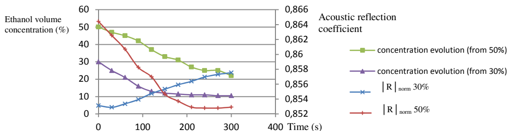
Fig. 2. Evolution of the concentration of ethanol (and of the acoustic reflection coefficient) in a 5 \mu\text{L} droplets of original volume concentrations 30% and 50%
