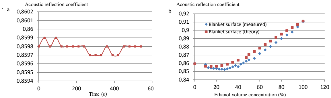
Fig. 1. Acoustic reflection coefficient |R|_{norm} : a) measured for water (21°C) as a function of time ; b) calculated and measured in ethanol/water mixtures as a function of Ethanol Volume Concentration .
