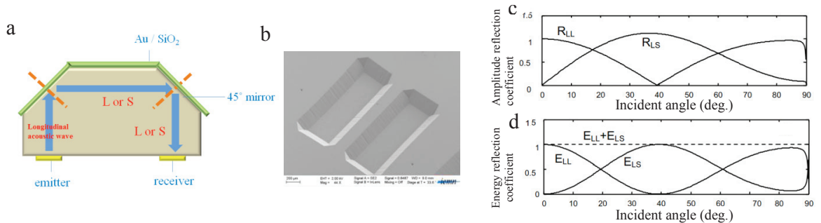
Fig. 1. a) Scheme diagram of the microsystem; Reflection coefficient of LL mode for longitudinal converted to longitudinal wave and TL mode for longitudinal to shear wave, for a longitudinal wave incidence at silicon-vacuum interface; b) SEM image of the cross-section of the 45^\circ mirrors; c) in amplitude and d) in energy. (ultrasonic characteristics of silicon : V_L = 8457 m/s; V_T = 5887 m/s)
