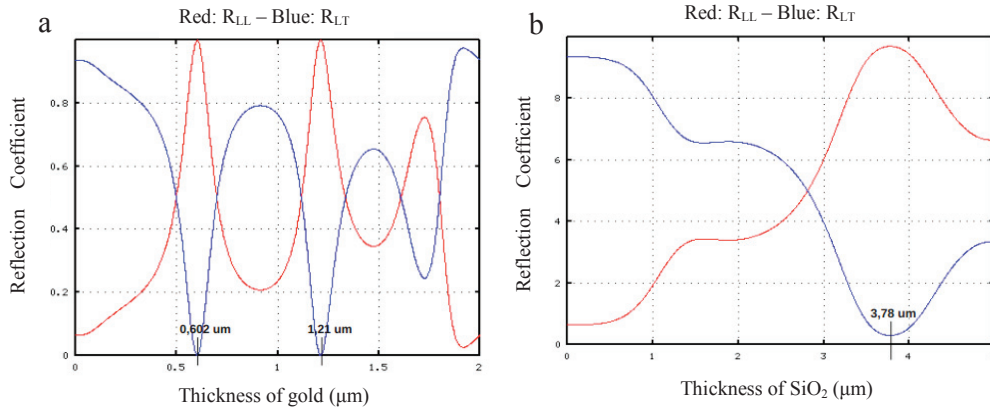
Fig. 2. Simulation of the reflection coefficient from longitudinal wave to shear wave for an incidence angle of 45^\circ and a central frequency of 1 GHz: a) Reflection coefficient with Au coating layer and b) with \text{SiO}_2 deposited on mirror surfaces. Red line is the reflection coefficient from longitudinal wave to longitudinal wave, and blue line indicates longitudinal wave converted to shear wave.
