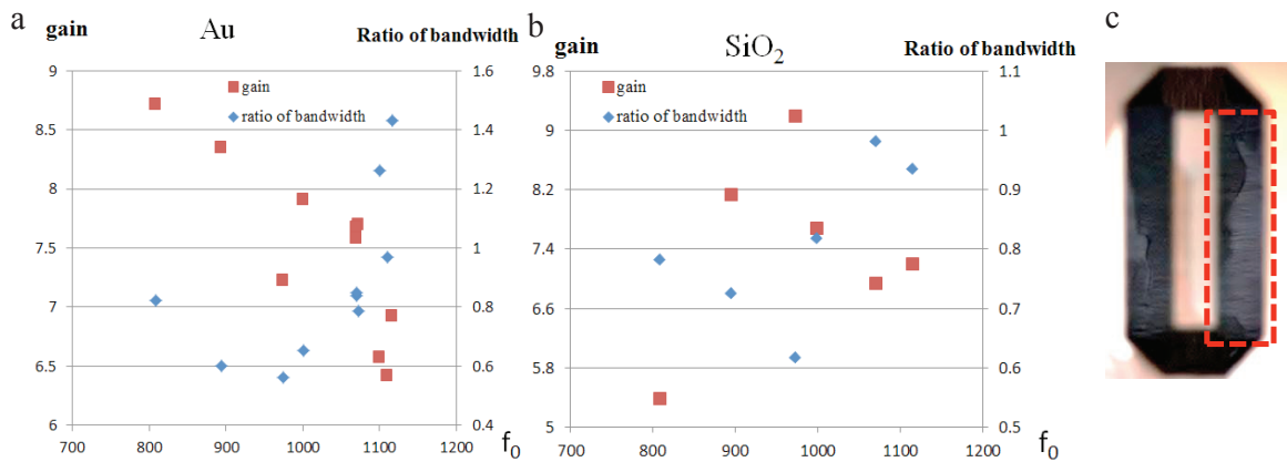
Fig. 3. Gain and bandwidth ratio comparison: a) with 800 nm gold layer introduction; b) with 3.8 \mu m SiO 2 layer; c) SiO 2 film partially lift-off. f_0 is the experimental central frequency of transducer.
