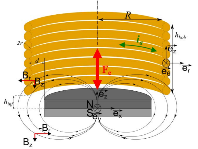
Figure 2: Diagram of the electromagnetic actuator with the different parameters and a view of the field lines
