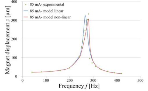
Figure 10: Comparison of MTL-system response between experimental results (green dots), linear simulation (blue line) and non-linear simulation (red line)
