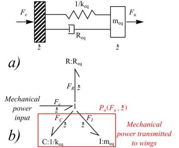
Figure 5: (a) Representation of the mechanical resonator (a) through a spring-mass representation, (b) through Bond Graph formalism
