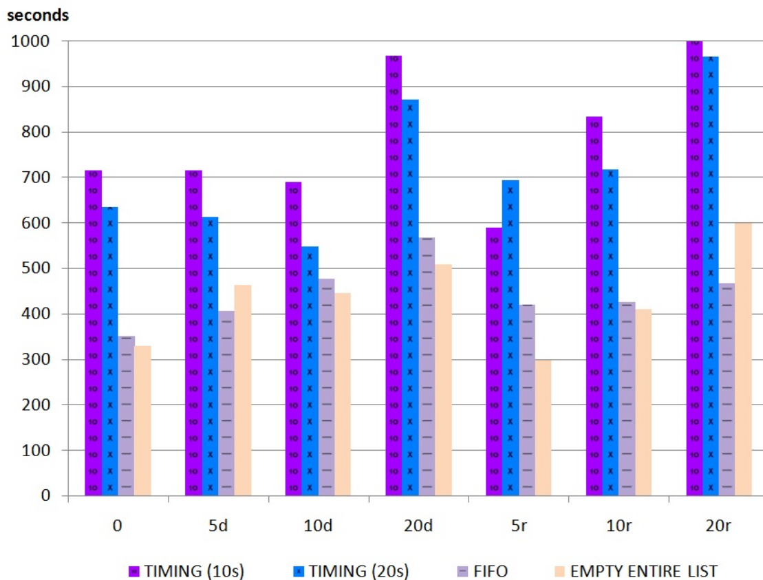
Figure 9: Results of various simulations on an area of the city of Valenciennes
