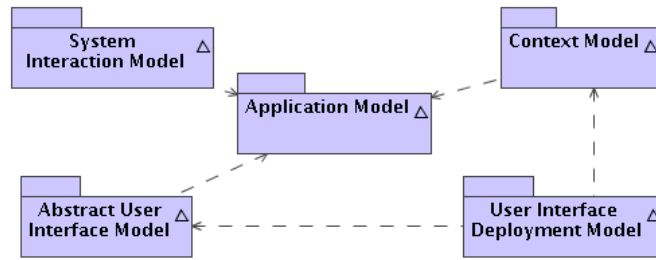
Figure 4. Overview of the models supported by UML Profile CUP 2.0
