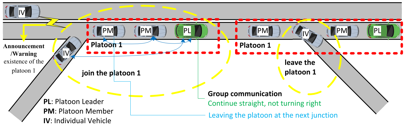
FIGURE 4. Vehicle platooning scenario shows the Join/Leave, Announcement/Warning and Group communication aspects.
