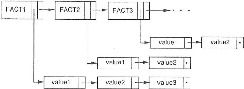
Fig. 3. The facts data base
