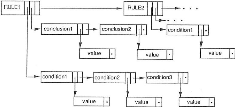
Fig. 4. The rules database
