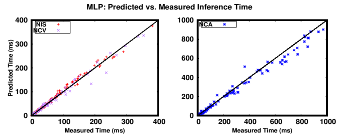
Fig. 9: Predicted vs. Measured Inference Time for MLP (AGX).
