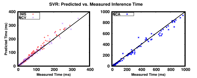
Fig. 7: Predicted vs. Measured Inference Time for SVR (AGX).
