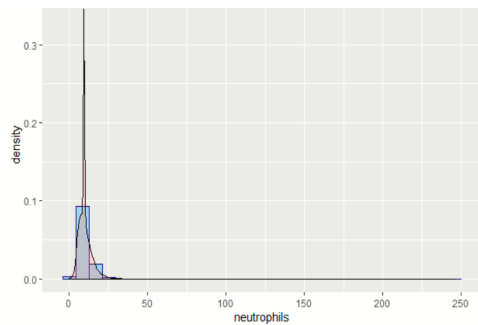
Fig. 1. Histogram before transformation.
