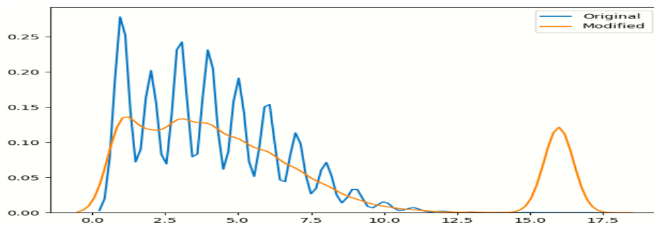
Fig. 5. SMOTER method for the variable LoS.
