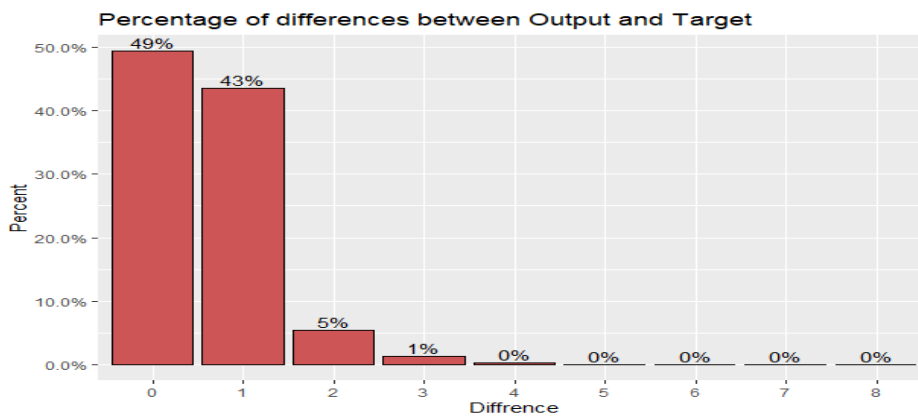
Fig. 6. Difference between output and target values.
