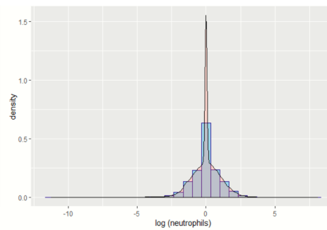
Fig. 2. Histogram after transformation.
