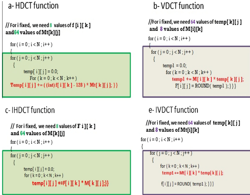
Fig. 12. DCT and IDCT functional decomposition.
