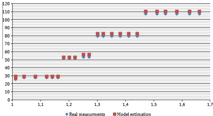
Fig. 13. Area usage (y axis) of the MIP model for the generated configurations for different speedups. The speedups are calculated relative to the configuration with 8 processors without HW accelerators.
