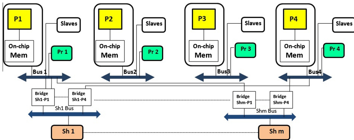
Fig. 2. Example of a SHt-MPSoC architecture with 4 processors. Each processor has one private HW accelerator (Pr i ) and share m accelerators (Sh i ) with the other processors.
