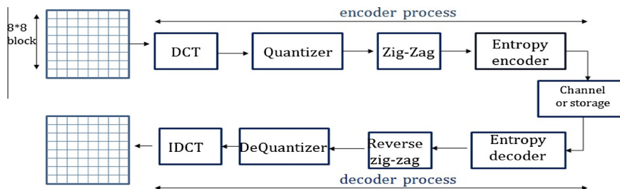
Fig. 11. Jpeg encoder and decoder tasks.
