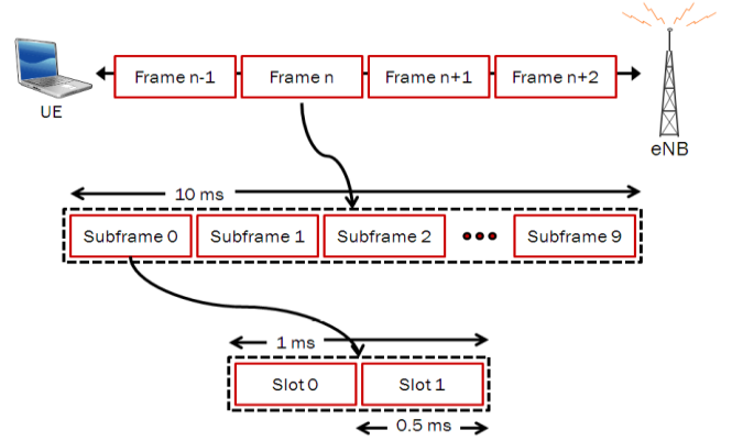
Fig. 5. LTE time-domaine structure
