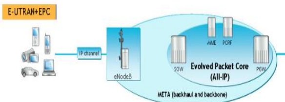
Fig. 1. LTE Architecture
