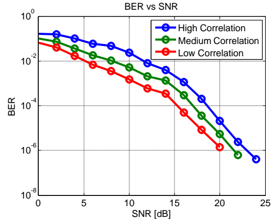
Fig. 8. BER vs SNR compared High Correlation, Medium Correlation and Low Correlation (T2X Communication)
