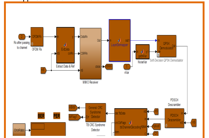
Fig. 6. LTE-Receiver Part
