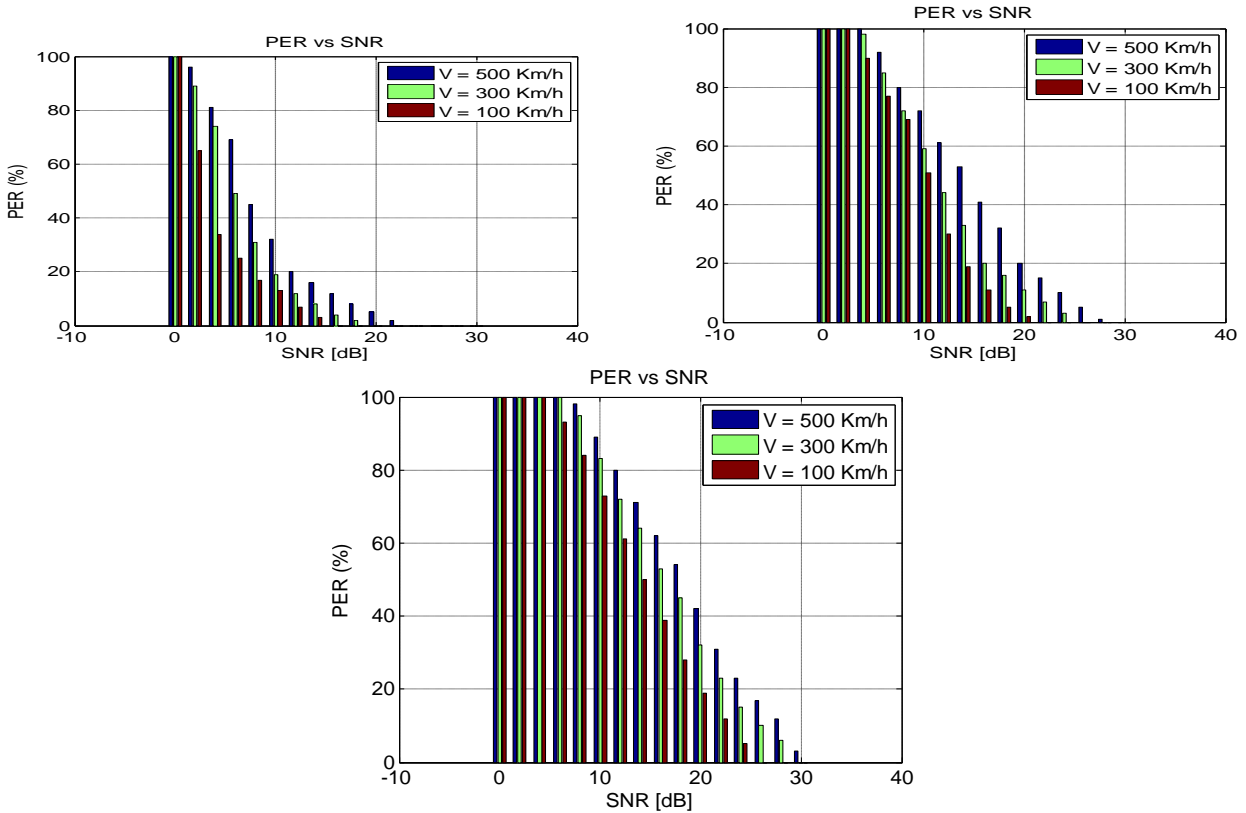
Fig. 14. PER vs SNR compared Mobile Velocities and Modulations (T2X Communication): a) QPSK, b) 16QAM, c) 64QAM
