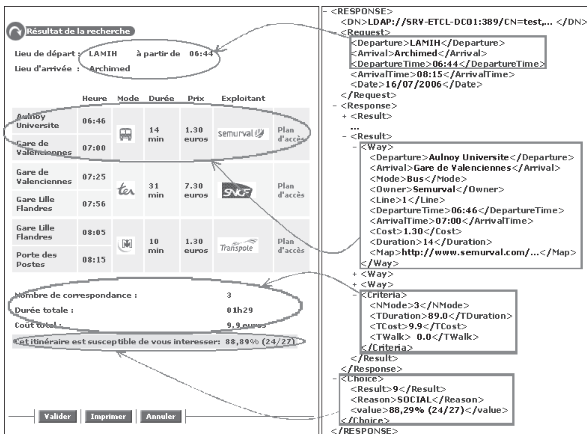
Figure 3.22. Use of data coming from PerSyst by itinerary search service
