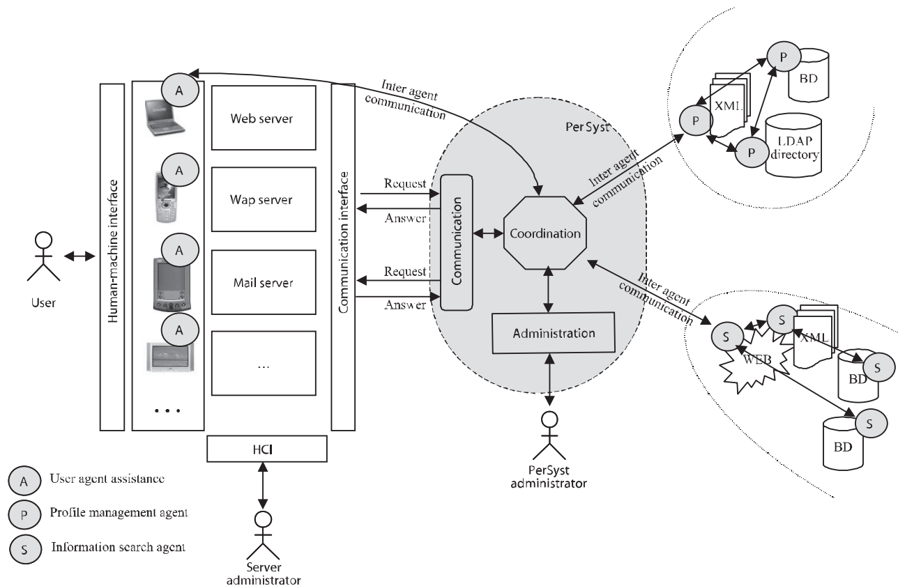
Figure 3.2. General architecture of PerSys
