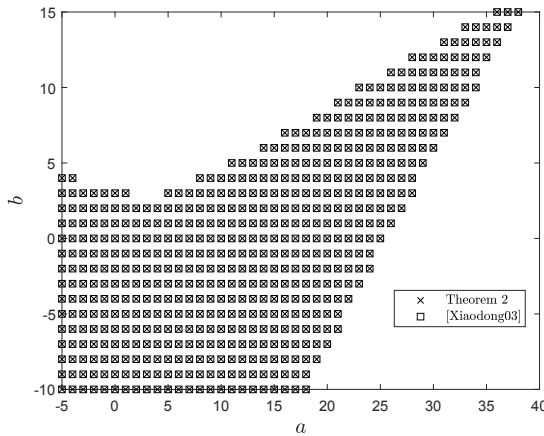
Fig. 3. Comparison between Theorem 2 and Lemma 4.
