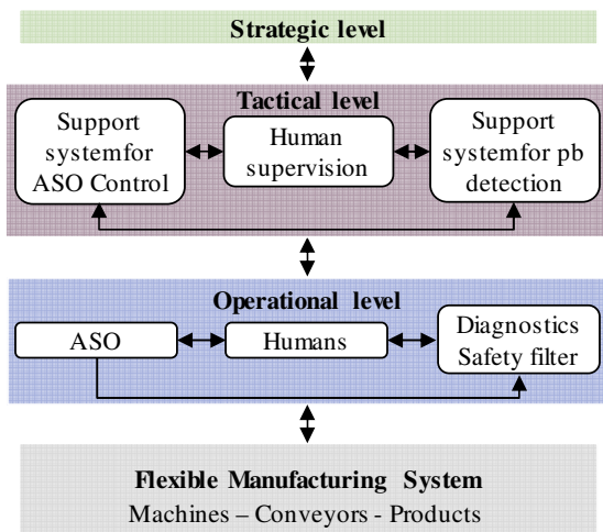
Fig. 3. Multi-level cooperation between Humans and innovative autonomous systems
