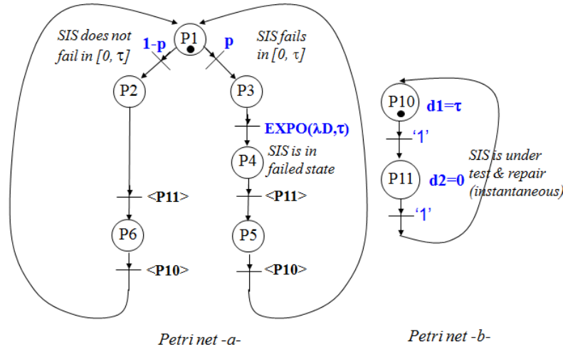
Figure 6. Reference model based onto a Stochastic P-temporized Petri Net for a 1oo1 SIS architecture
