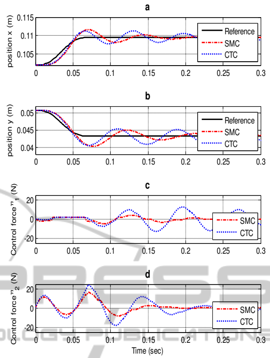
Figure 5: Control schemes for low trajectory (T1) and \Delta m = 0.816 .
