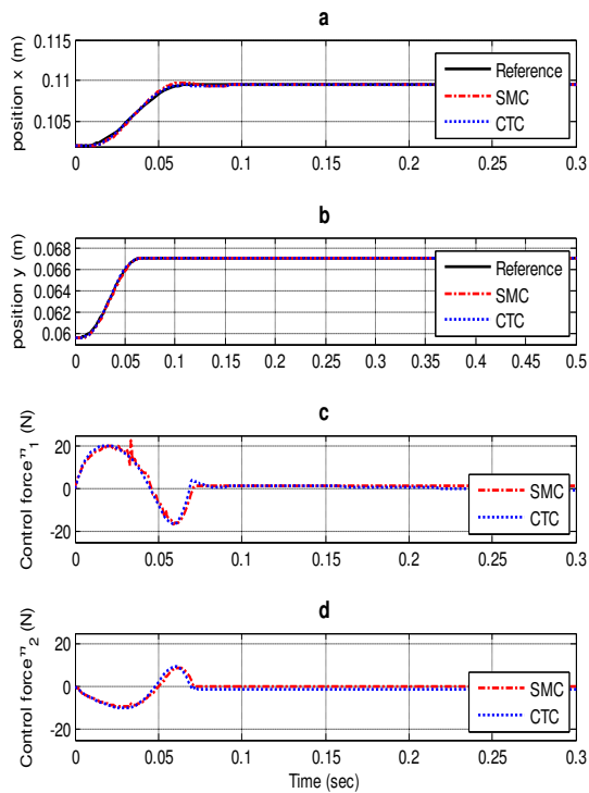
Figure 4: Control schemes for high trajectory (T2) and \Delta m = 0 .
