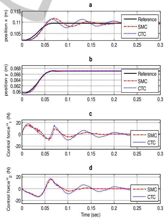
Figure 6: Control schemes for high trajectory (T2) and \Delta m = 0.816 .
