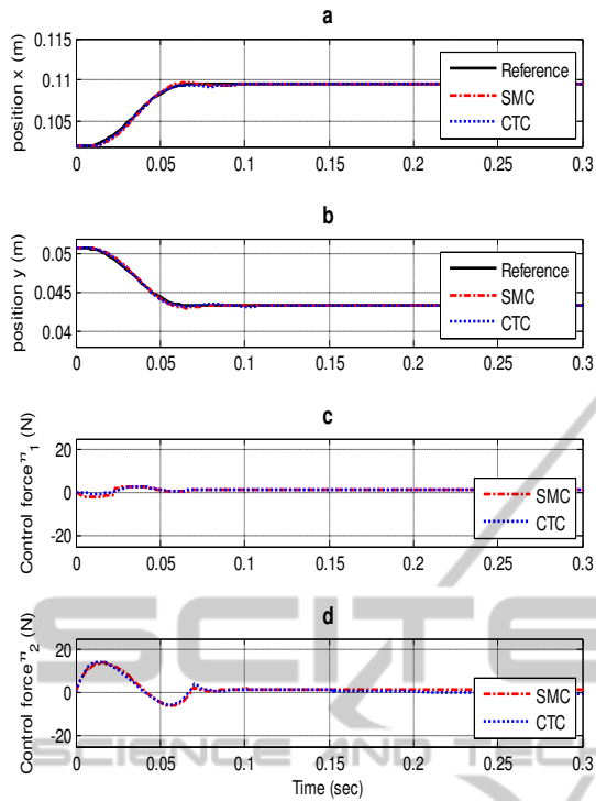
Figure 3: Control schemes for low trajectory (T1) and \Delta m = 0 .
