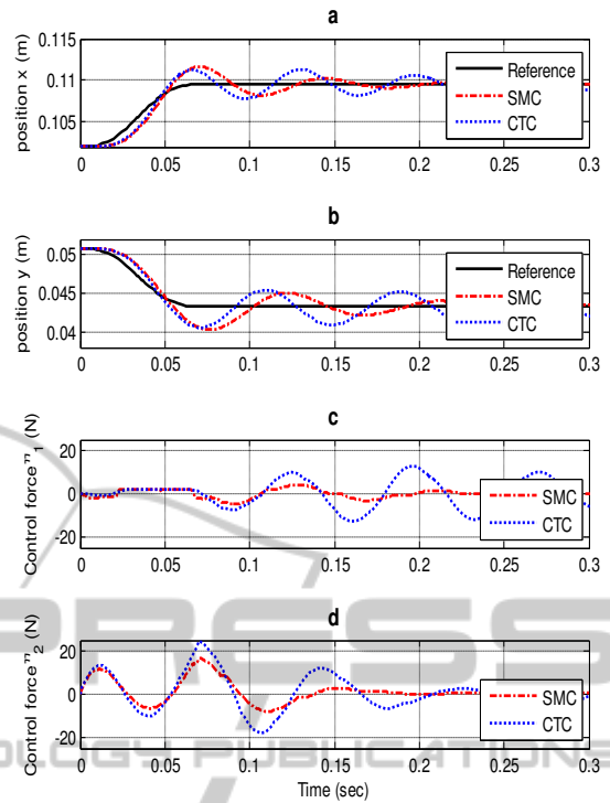
Figure 5: Control schemes for low trajectory (T1) and \Delta m = 0.816 .
