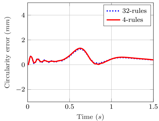
Fig. 4 Circularity errors in Case 1 obtained with 32-rules controller (dotted blue), with 4-rules controller (solid red).
