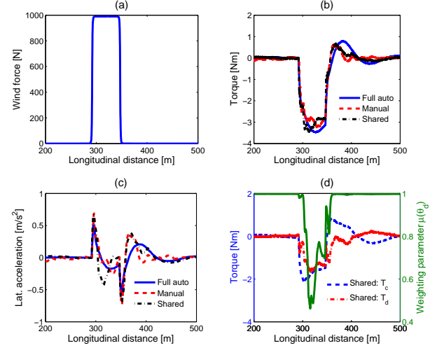
Fig. 10. Disturbance rejection performance for three cases: (1) full automatic control, (2) manual control, (3) shared control.
