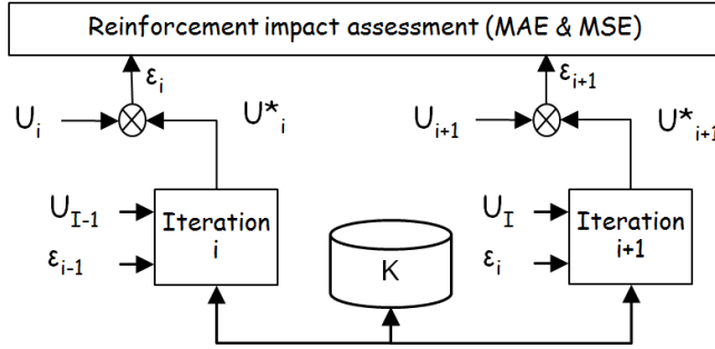
Figure 2: The generic hybrid learning system architecture.
