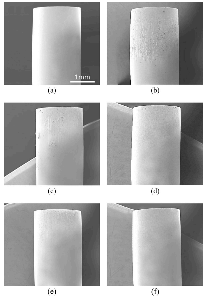
Fig. 4. SEM micrographs of the punch surface of (a) a new punch and (b-f) punches after testing with different lubricants: (b) DB 4265, (c) Drosera MS 5, (d) Pn226, (e) SF125 and (f) TDN81.
