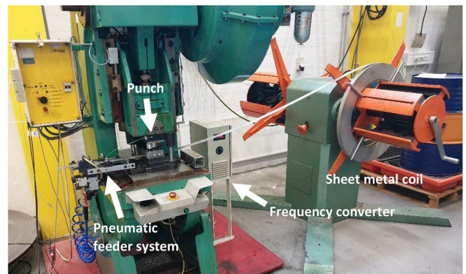
Fig. 1. Eccentric press equipped with punching tool, feeder system and a load cell for measurement of the punch force and the backstroke force.
