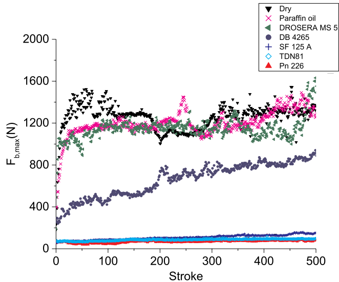
Fig. 3. Backstroke force as function of number of strokes for the tested lubricants and under dry conditions.
