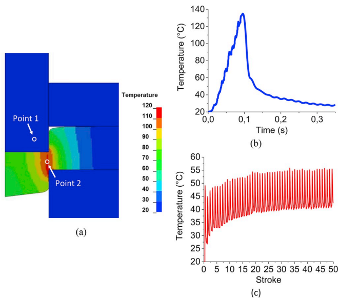
Fig. 8. Thermo-mechanical FE simulation of temperature showing (a) the temperature distribution in the tools and workpiece, (b) temperature development in point 2 during stroke number 1, and (c) temperature development in point 1 during the first 50 strokes.
