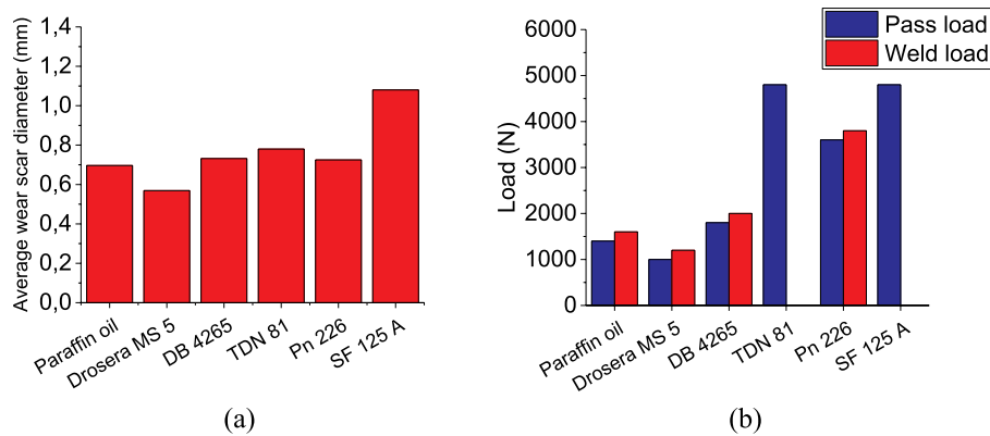
Fig. 5. Characterization of the wear behavior and the load bearing capacity of the tested lubricants in the four-ball test. The results are shown by (a) developed wear scar diameter and (b) weld load and pass load.
