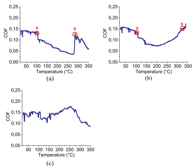
Fig. 6. COF as a function of the test temperature in pin-on-disc testing with (a) Pn226, (b) Drosera MS 5 and (c) Paraffin oil.
