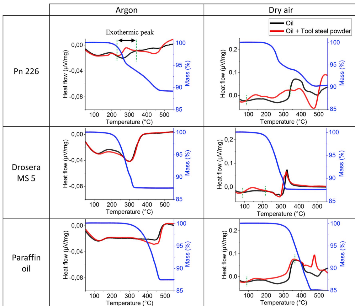
Fig. 7. TG/DTA thermograms of the tested lubricants.
