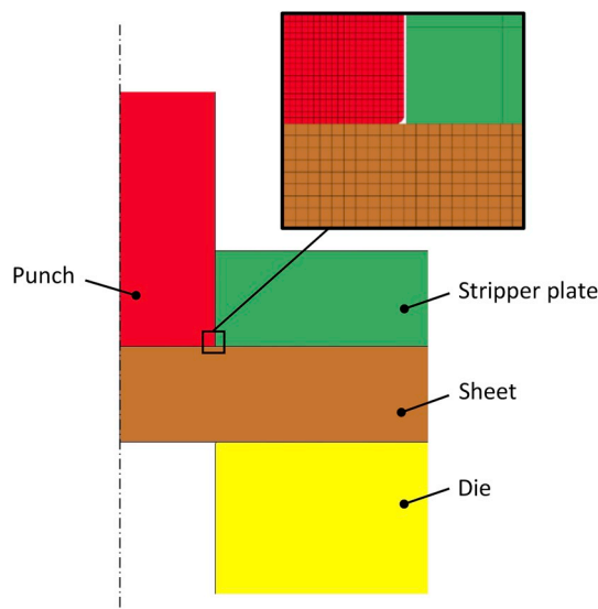
Fig. 2. Numerical model with initial mesh shown around the punch corner in the detail.
