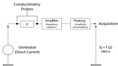
Fig. 6. Simplified diagram of the conductimetry method.
