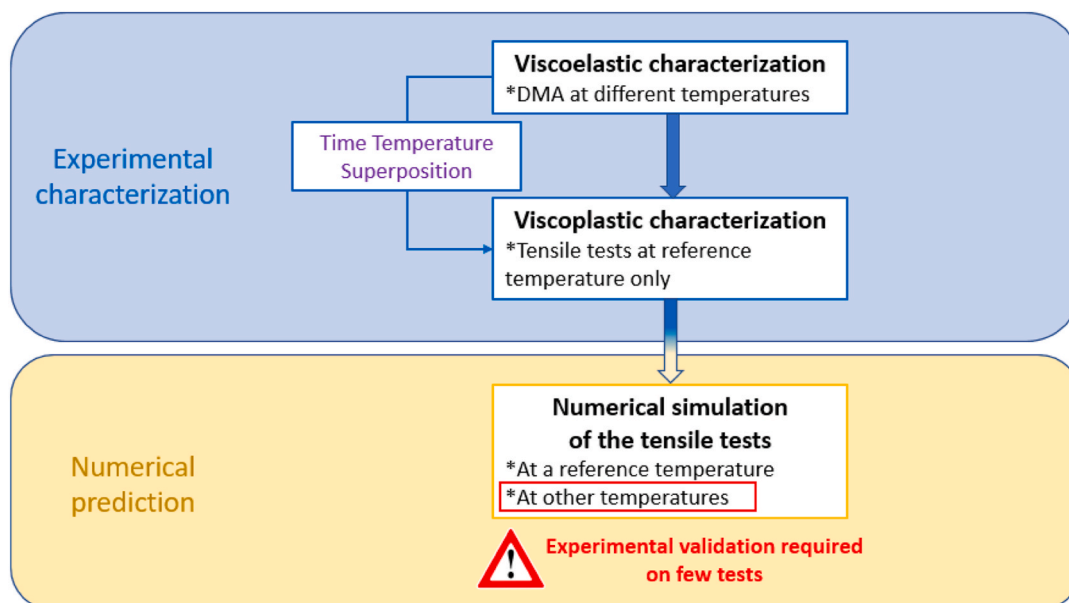
Fig. 17. New characterization procedure for a semi-crystalline polymer for a wide strain rate range and temperature.
