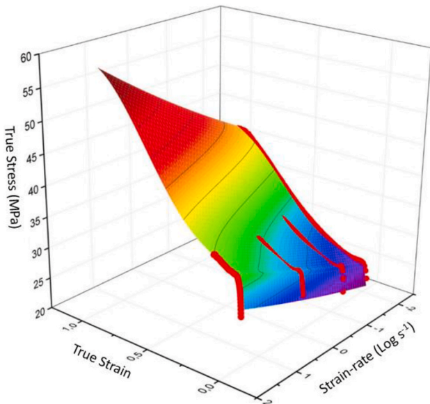
Fig. 10. Behaviour surface obtained by the SEE Method at +23 °C.
