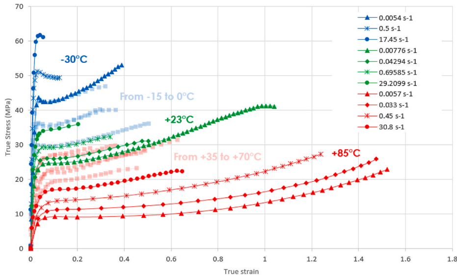
Fig. 9. Tensile tests at different strain rate (from 5.10 to 3 s -1 to 30 s -1 ) and temperature (from -30 °C to +85 °C).
