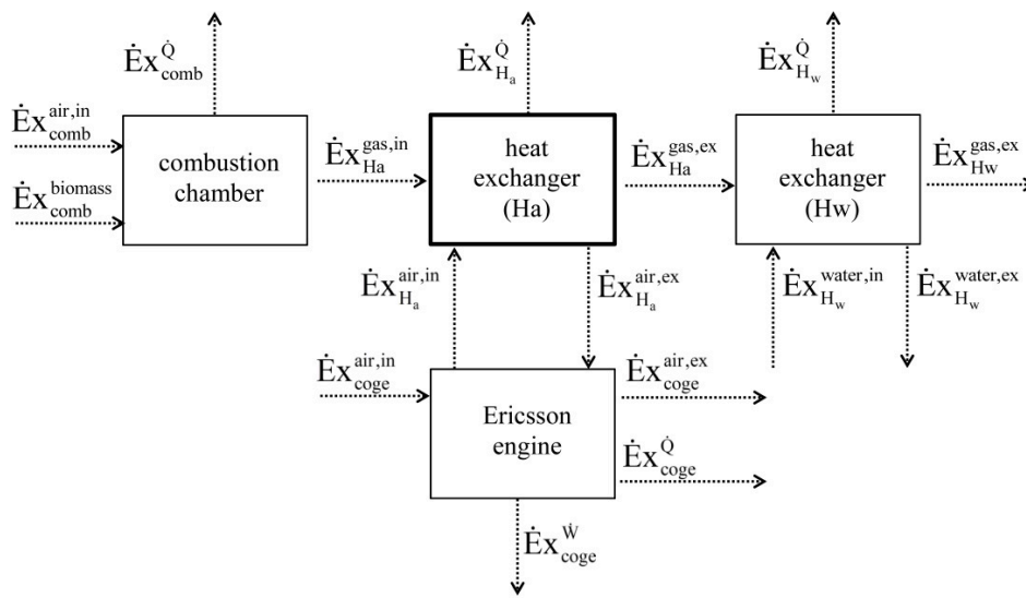
Figure 8. Exergy exchanges in the solid biomass-fueled micro-CHP system.
