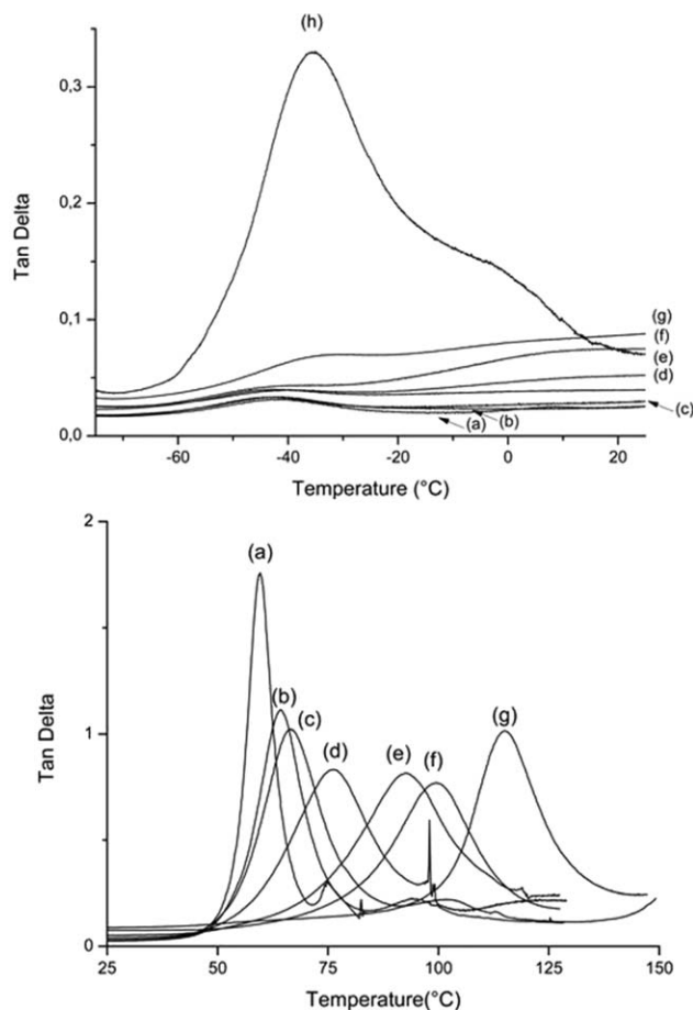
Figure 2. \tan\delta curves of (a) PLA/BS, (b) PLA80/PMMA20/BS, (c) PLA70/PMMA30/BS, (d) PLA50/PMMA50/BS, (e) PLA30/PMMA70/BS, (f) PLA20/PMMA80/BS, (g) PMMA/BS, (h) neat BS.
