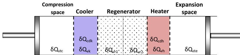
Fig. 5. Location of the various energy losses in a Stirling engine.
