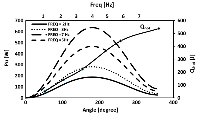
Fig. 8. Output brake power and heater energy for one Stirling cycle vs. engine frequency.
