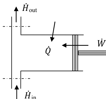
Figure 3. Control volume.
