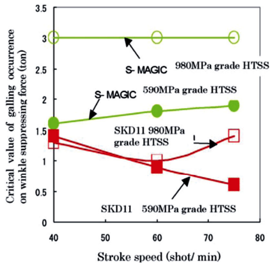
Fig. 14 Anti-galling tool steel for sheet forming. Reproduced with permission from Ref. [57], © Elsevier B.V. 2011.
