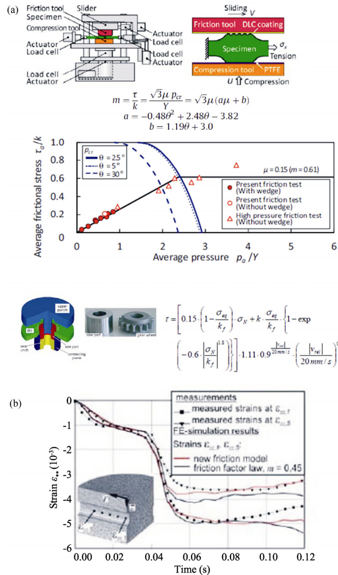
Fig. 17 Friction model for metal forming. (a) Relating to pressure and surface condition. Reproduced with permission from Ref. [75], © CIRP. Published by Elsevier Ltd. 2014. (b) Relating to slip rate and heat transfer. Reproduced with permission from Ref. [76], © Elsevier B.V. 2004.
