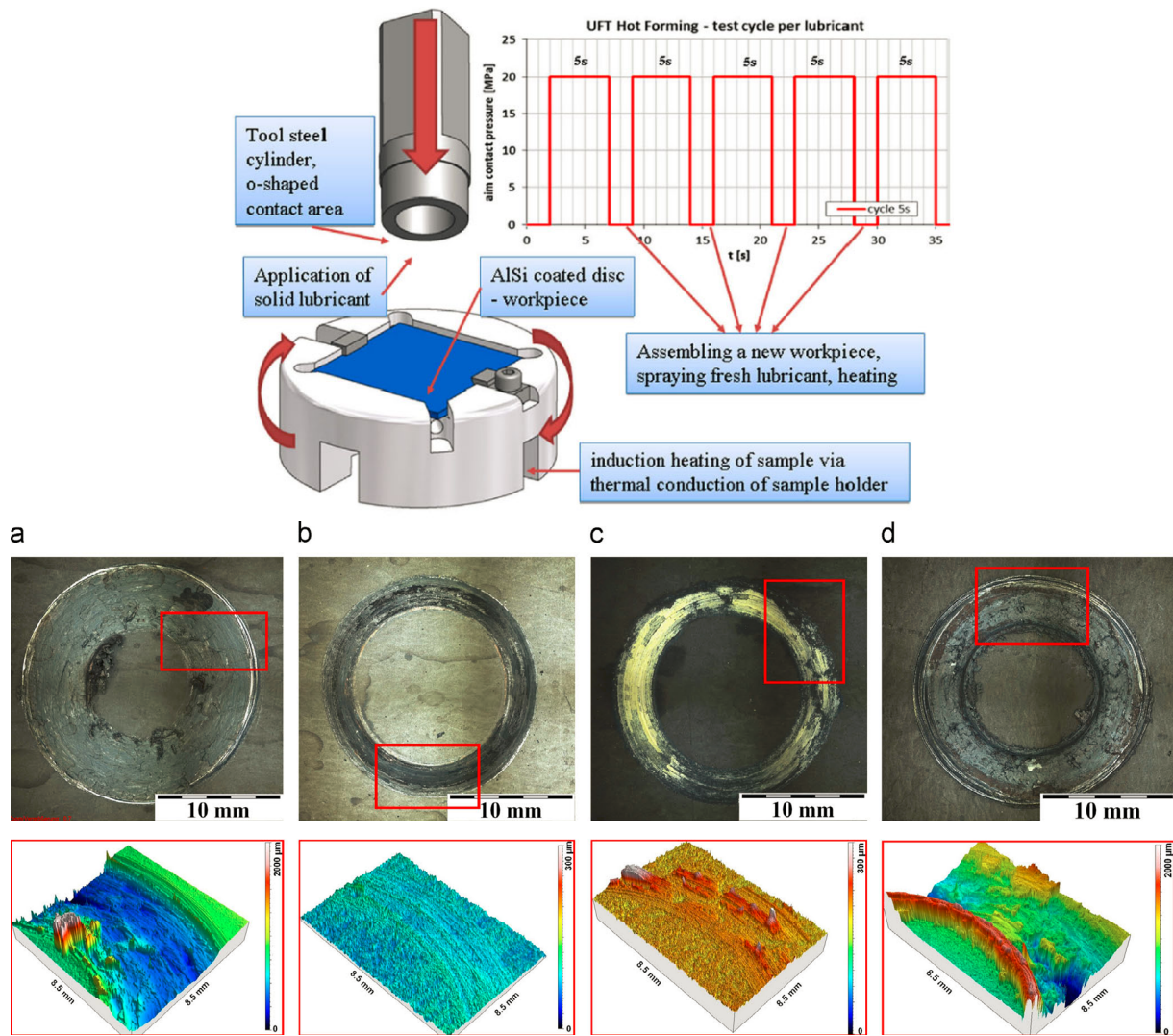
Fig. 10 Lubricant evaluation at elevated temperatures. Reproduced with permission from Ref. [43], © Elsevier Ltd. 2014.
