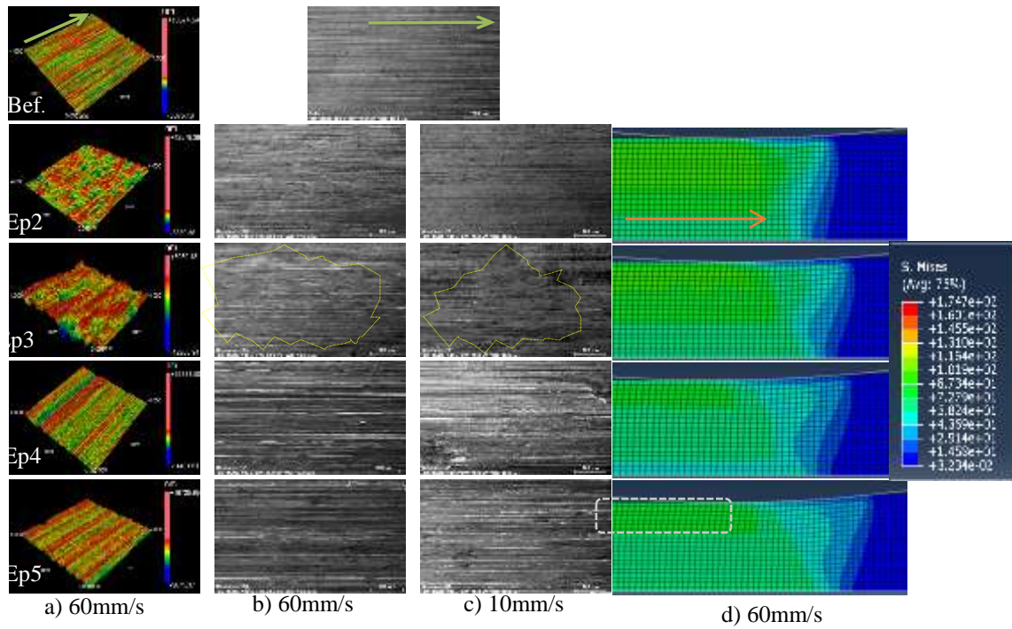
Figure 8. Effect of cold forging of aluminum alloy on the surface integrity
