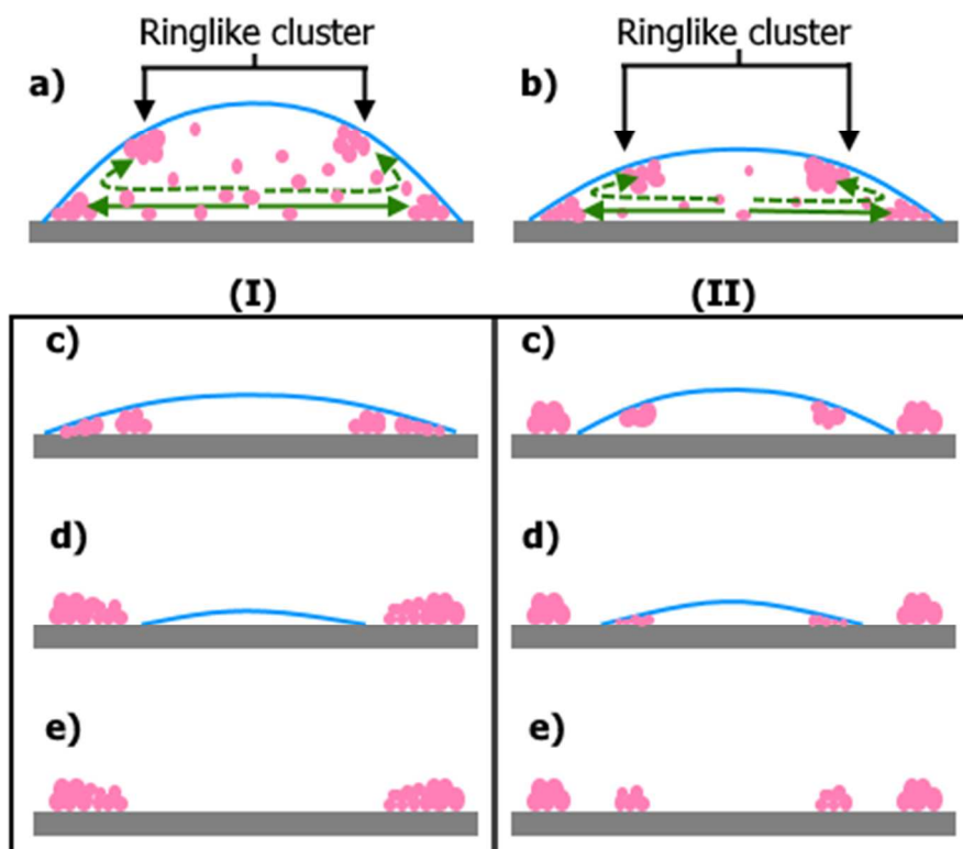
Figure 8. Sketch of the internal flow pattern inside an evaporating water-based bi-disperse drop containing a mixture of 3.2\ \mu\text{m} diameter particles and 1\ \mu\text{m} mean diameter particles onto a heated silicon substrate; The outward and temperature-dependent Marangoni flows are indicated by the solid and dashed arrows, respectively. The black bar indicates a stagnation point where the surface flow changes its direction.
