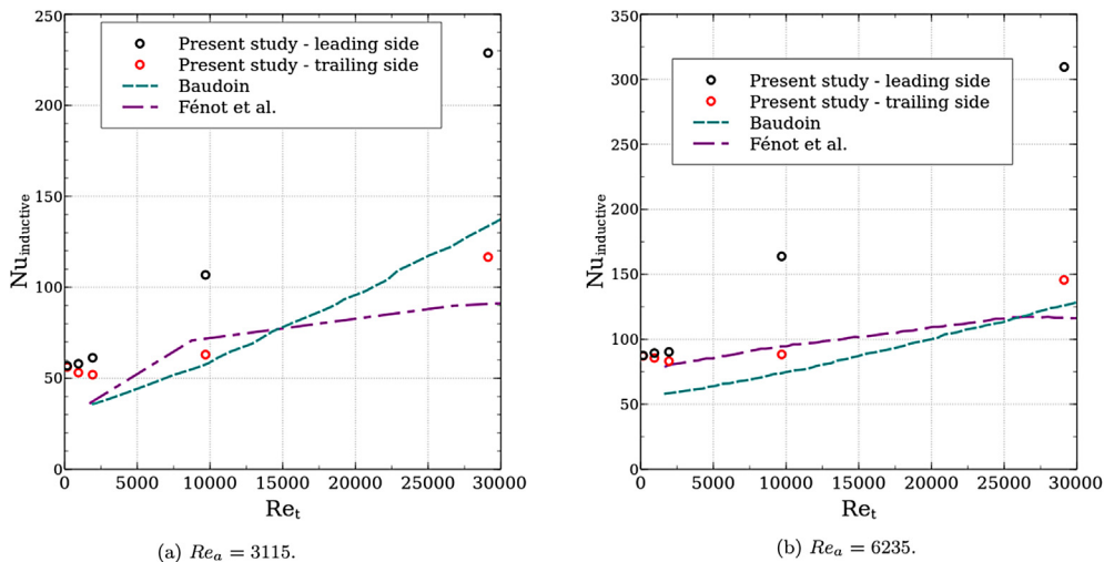
Fig. 13. Evolution of the Nusselt number in the inductive faces as a function of Re_t compared to a rotating tube ([3]) and a rotating slotted cylinder ([8]).
