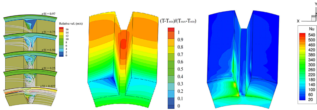
(a) Laminar with vortices ( Re_a = 779 , Re_t = 29130 ).
