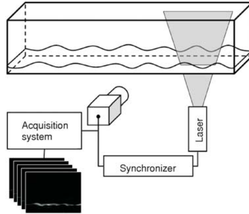
Figure 2. LeDaR method
