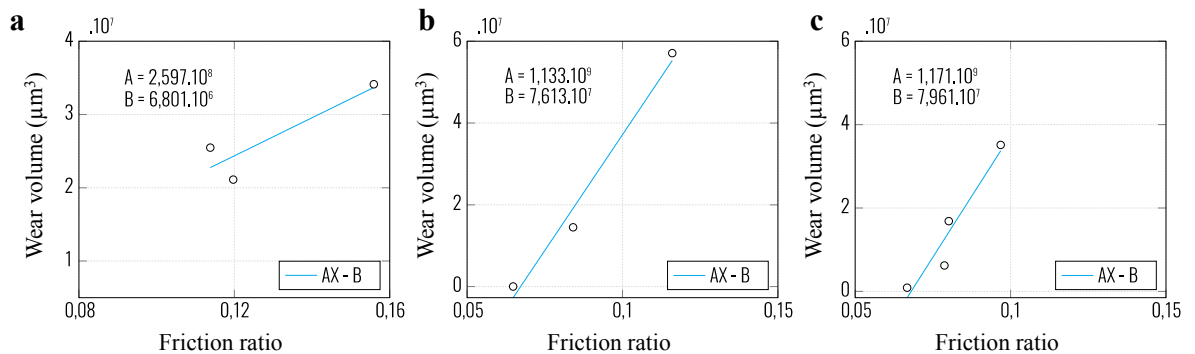
Fig. 5. Wear volumes as a function of the friction ratio (a) 20 mm.s -1 (b) 100 mm.s -1 (c) 200 mm.s -1 .
