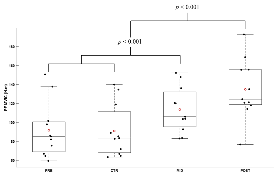
Figure 3. Average torque during MVIC in plantarflexion (N.m) according to the evaluation session (PRE, CTR, MID, POST sessions). Each whiskers box indicates the mean (red circle) and the median (horizontal line). The inferior edge and superior edges of the box indicate the 25th and 75th percentile, respectively. Error bars represent the most extreme and non-outlier data points. Black dots represent individual participant performance.
