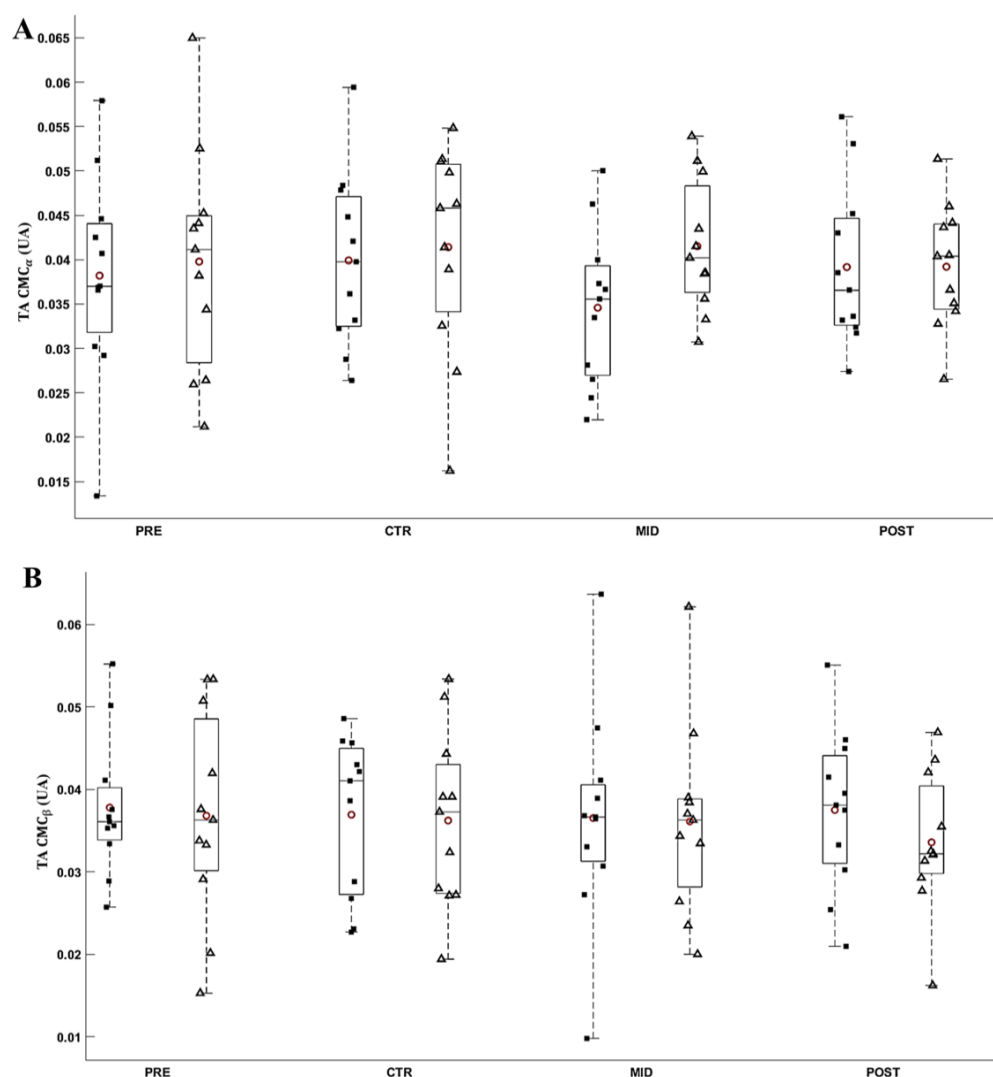
Figure 10. Average \alpha (A) and \beta (B) CMC_{TA} during submaximal contractions computed according to the torque levels, T_0 (black square) and T_i (white triangle), and evaluation sessions (PRE, CTR, MID, POST sessions). Each whiskers box indicates the mean (red circle) and the median (horizontal line). The inferior and superior edges of the box indicate the 25th and 75th percentile, respectively. Black dots represent individual participant performance. Error bars represent the most extreme and non-outlier data points.
